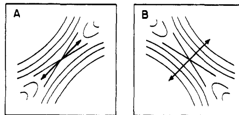
Figure 9. Level lines of constant energy that pass through the saddle point of an energy contour diagram. The level lines show where the curvature of the surface changes from negative to positive. A reaction coordinate is drawn to bisect the level lines, along the direction of negative curvature. The reaction coordinate may pass through a narrow col, A, or over a broad ridge, B.
